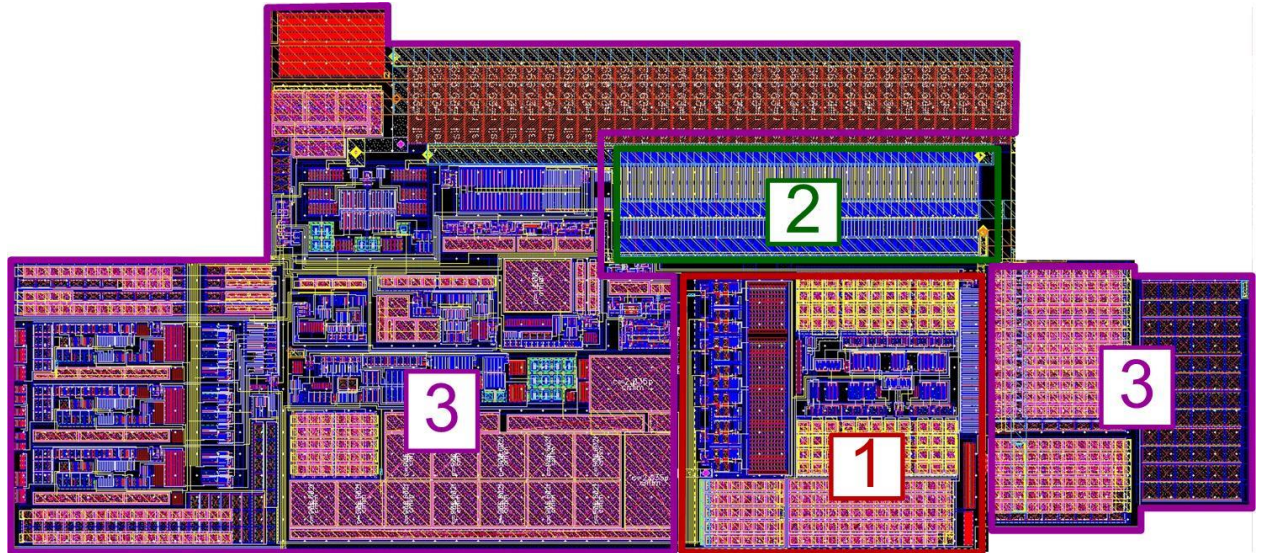
Figure 2: Power supply voltage stabilizer layout view
