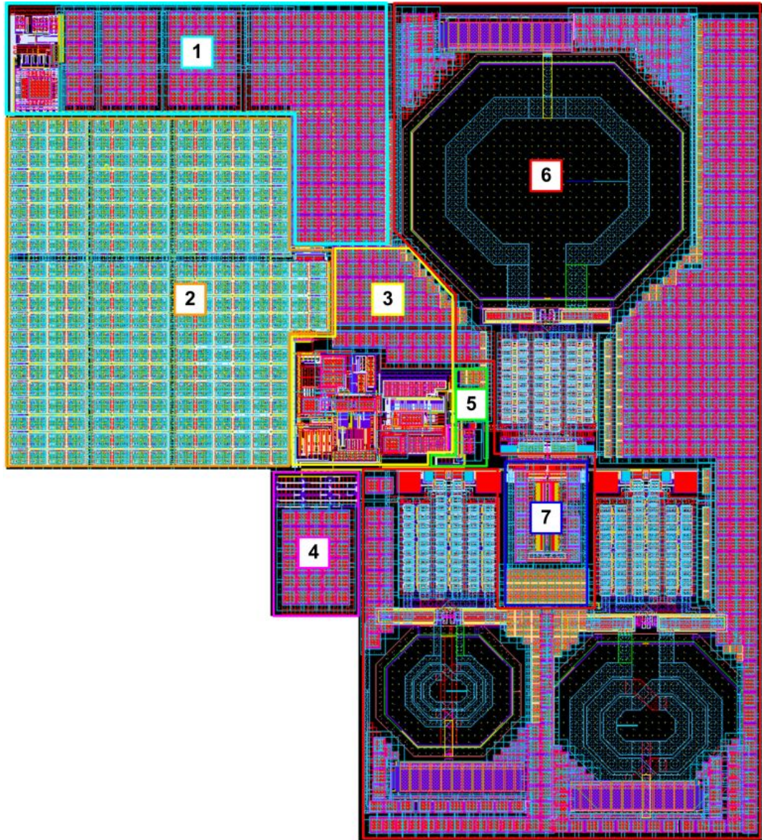
Figure 2: Device layout view.
