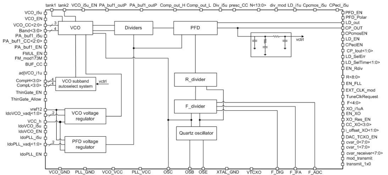
Figure 1: Phase-locked loop system structure.
